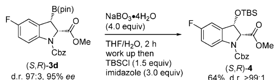
Scheme 3. Stereospecific oxidation of chiral 3-borylindoline (S,R)-3d .
